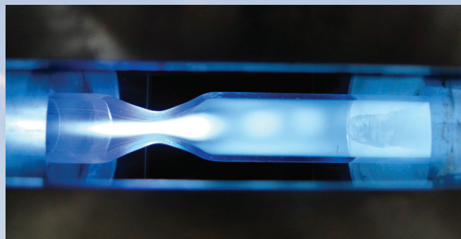
DIFFER / CO 2 plasmolysis reactor
